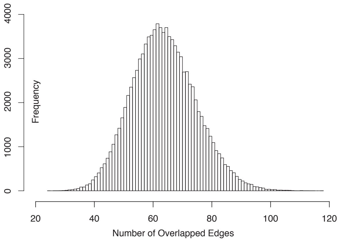
Fig. S2. Distribution of overlapped edges within distance 6 between the 527 network and the randomly substituted genome-wide network.
